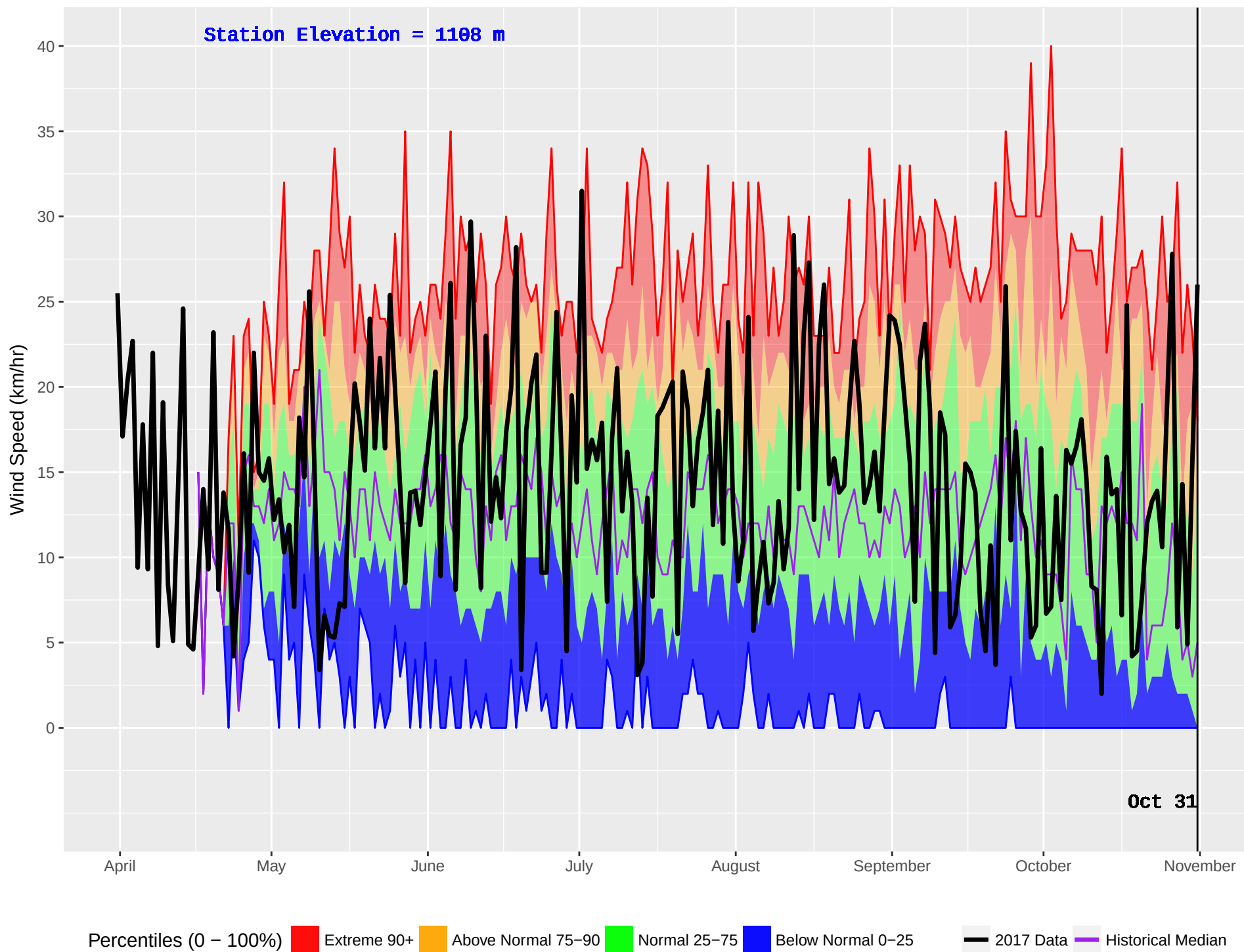
NABESHE (151) : Historical (1987–2016) and Current (2017) Noon Wind Speed
