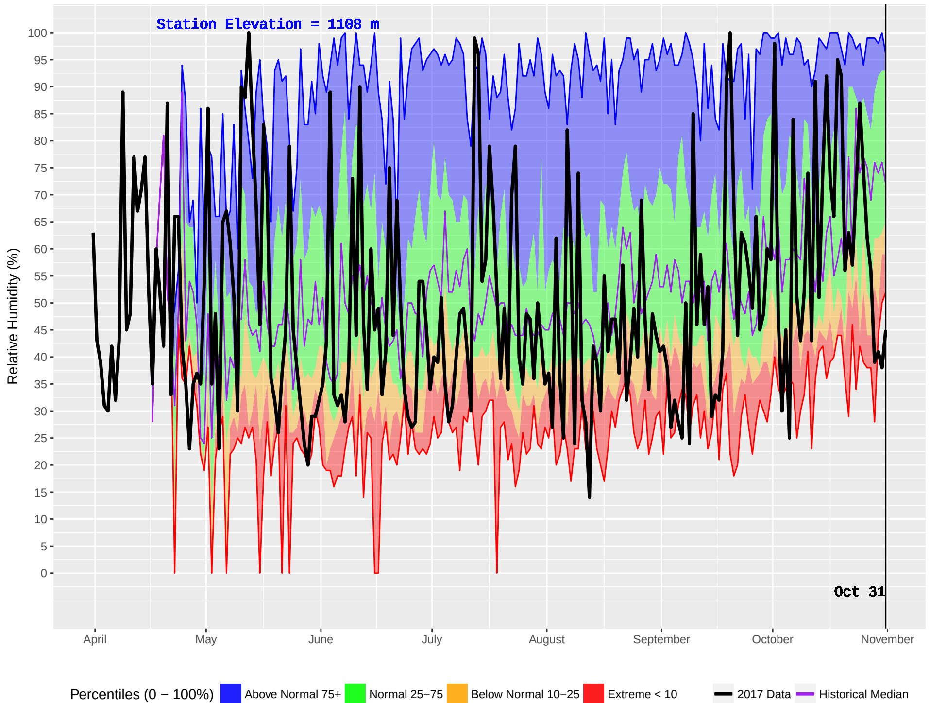
NABESHE (151) : Historical (1987–2016) and Current (2017) Noon Relative Humidity
