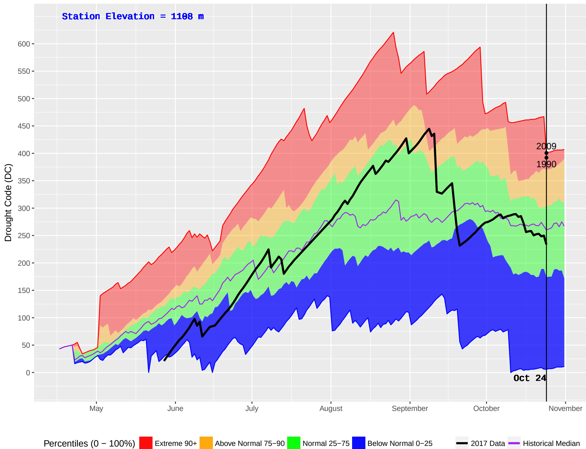
NABESHE (151) : Historical (1987–2016) and Current (2017) Noon Drought Code (DC)
