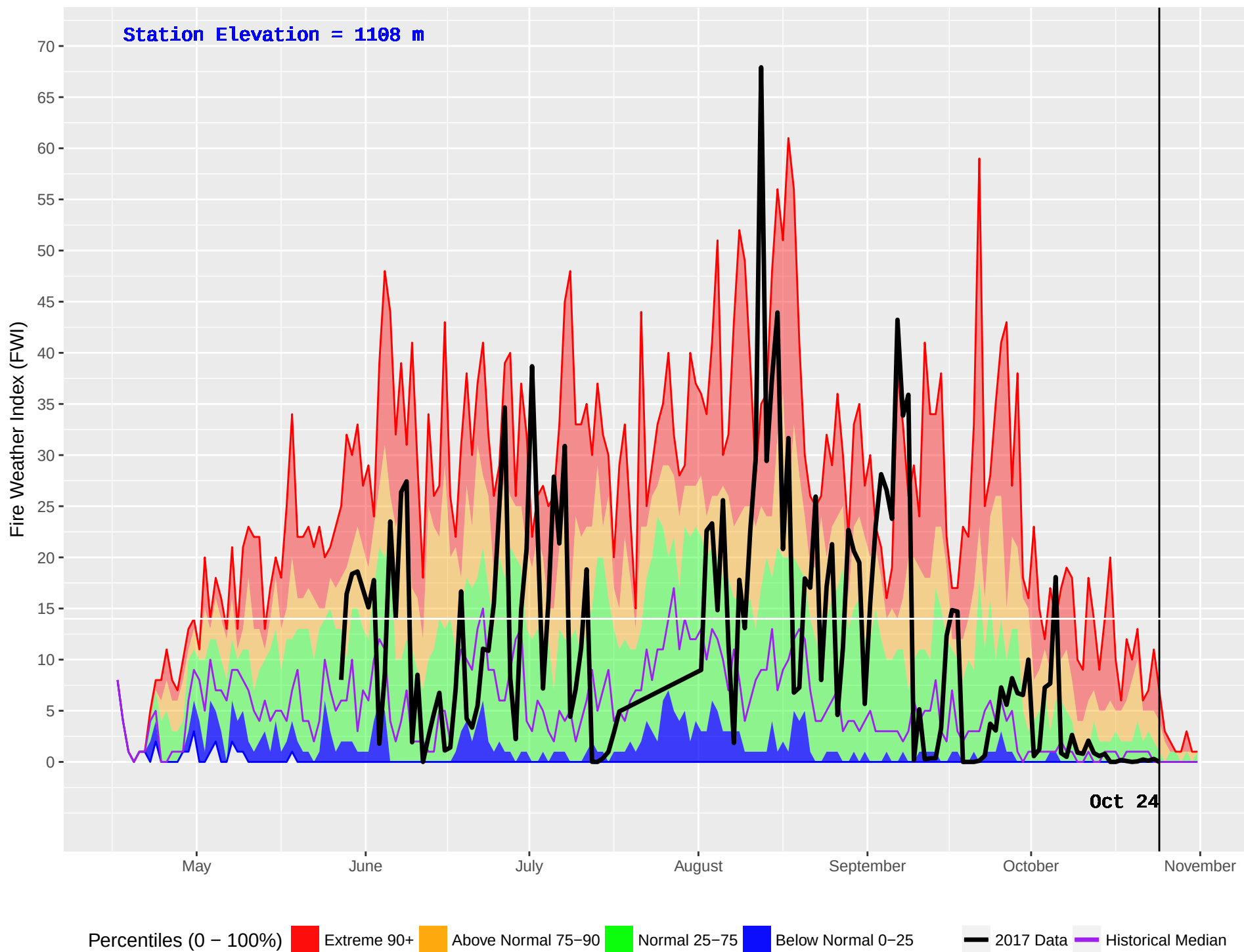
NABESHE (151) : Historical (1987–2016) and Current (2017) Noon Fire Weather Index (FWI)
