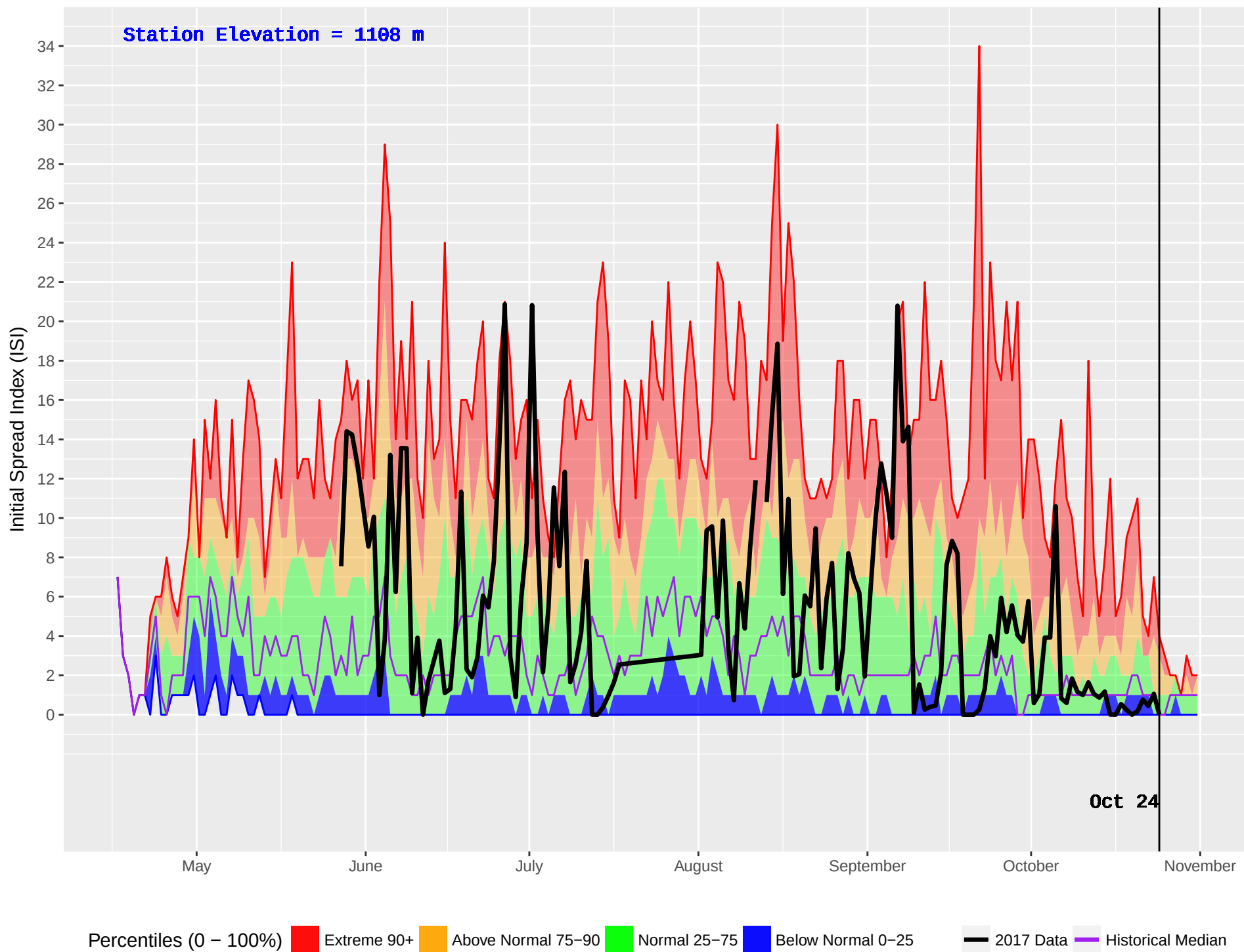
NABESHE (151) : Historical (1987–2016) and Current (2017) Noon Initial Spread Index (ISI)
