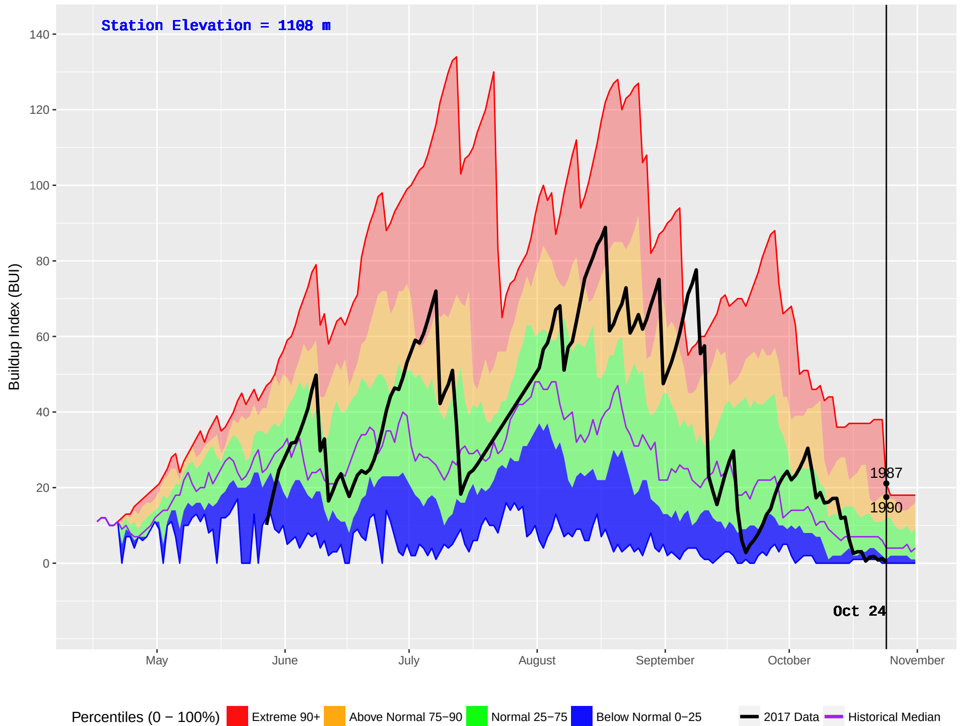
NABESHE (151) : Historical (1987–2016) and Current (2017) Noon Buildup Index (BUI)
